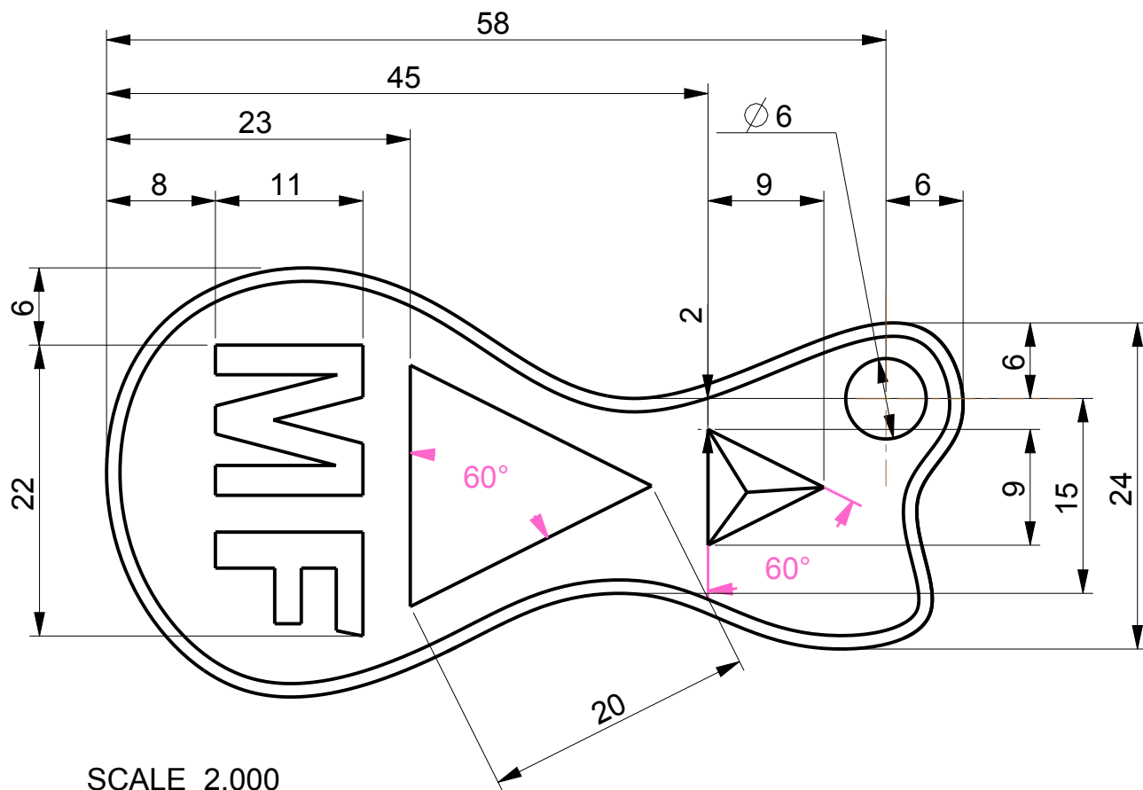
Key Fob drawn by Michael Franzen for Technical Design
